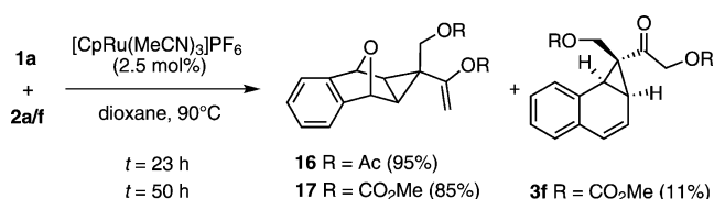
Scheme 4. Outcome of the coupling reaction according to the catalyst.
